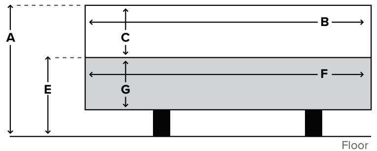
Fig 2. Side View
